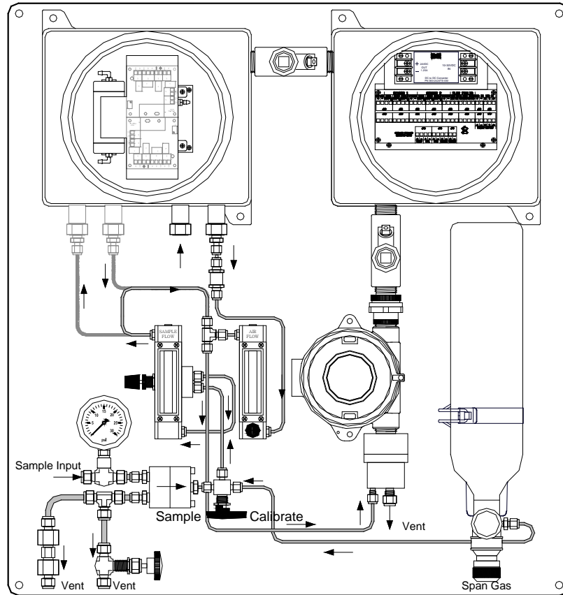
Figure 17 Unit Flow Diagram
