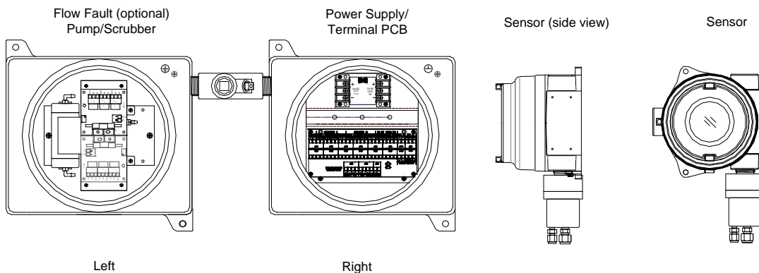
Figure 6 Enclosures
