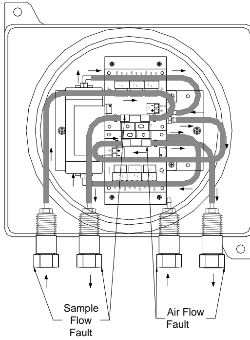
Figure 18 Pump Box Flow Diagram
