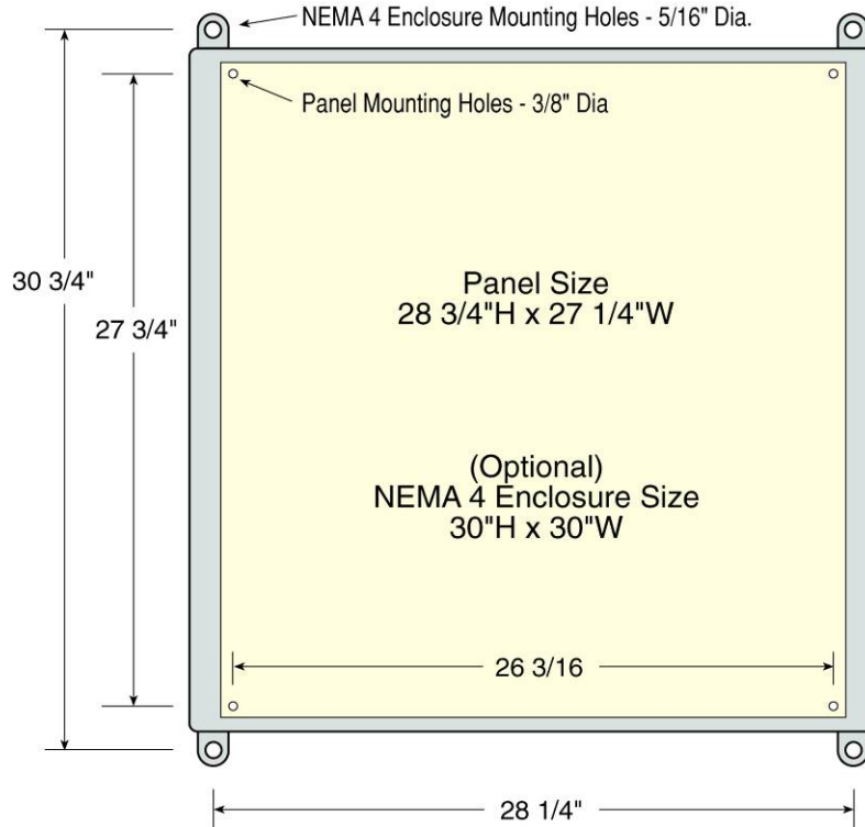
Figure 7 Unit Dimensions
