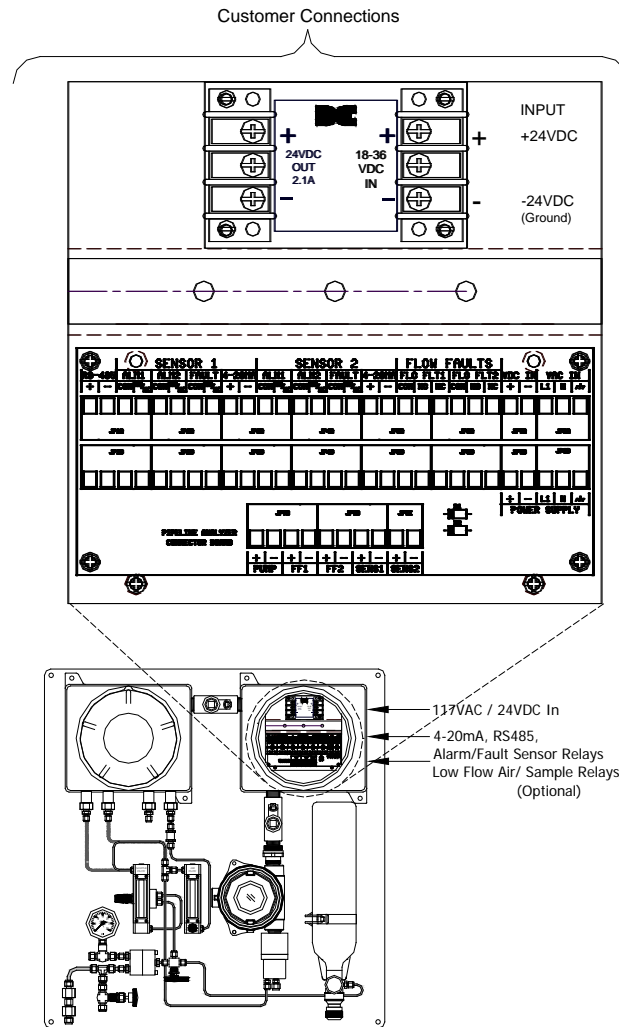
Figure 10 Installation Wiring Connections
