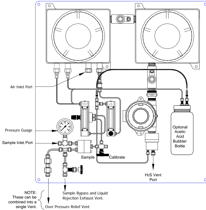
Figure 9 Optional Bubbler Bottle
