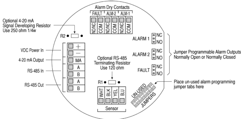
Figure 5 Connector Board Terminals
