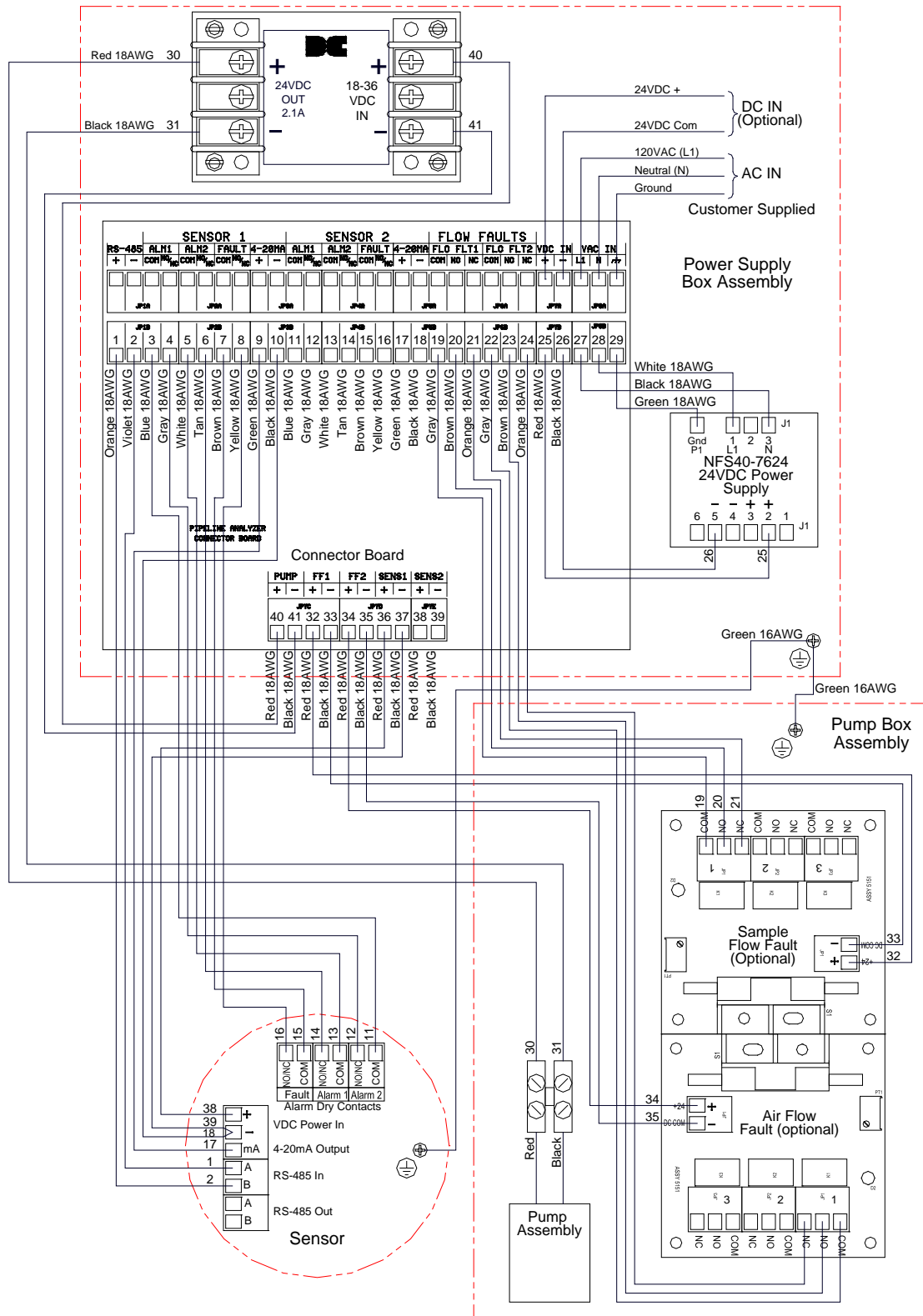
Figure 19 Wiring Diagram
