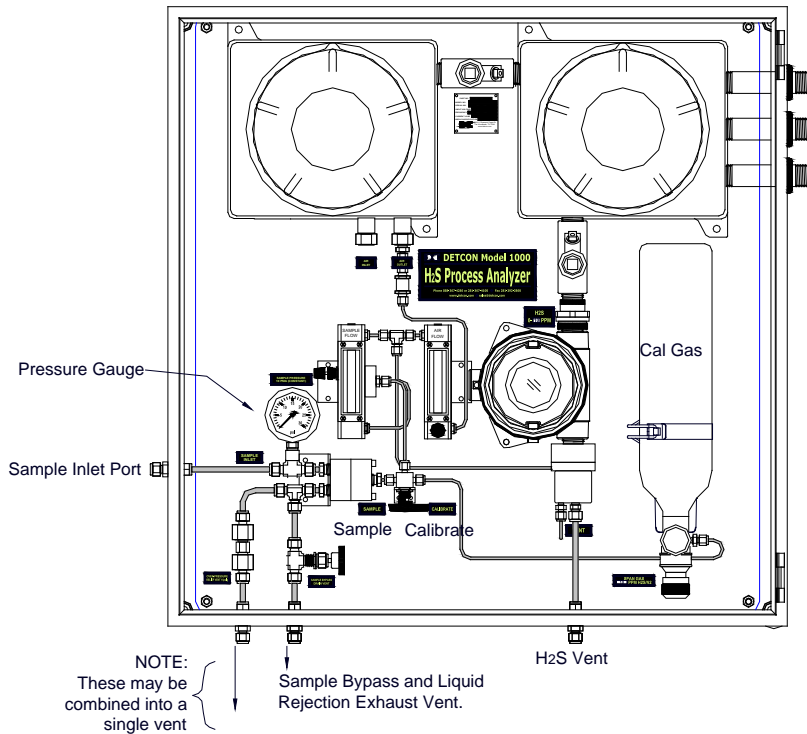
Figure 8 Port Identification
