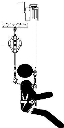
A Work Positioning or Controlled Descent, with Seat Sling
