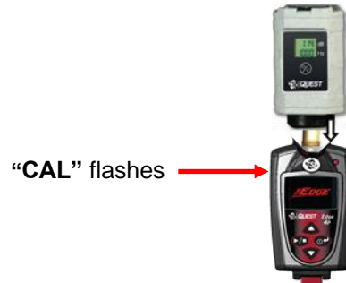
Figure 4-4 Calibrating
