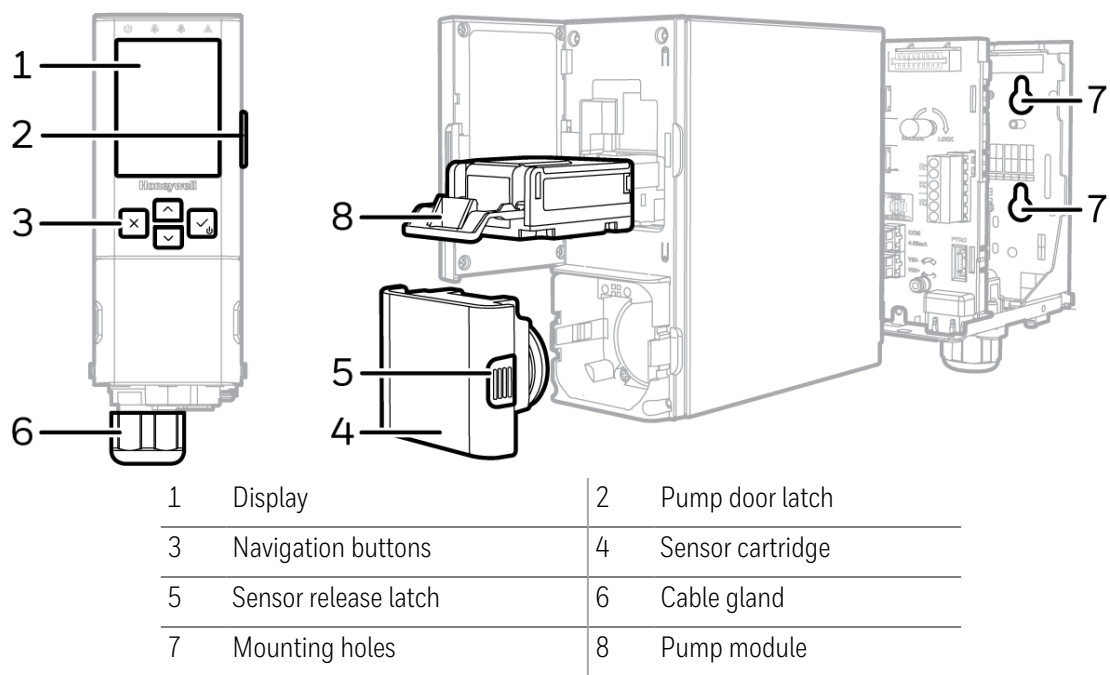
FIGURE 1 -1: Hardware components
