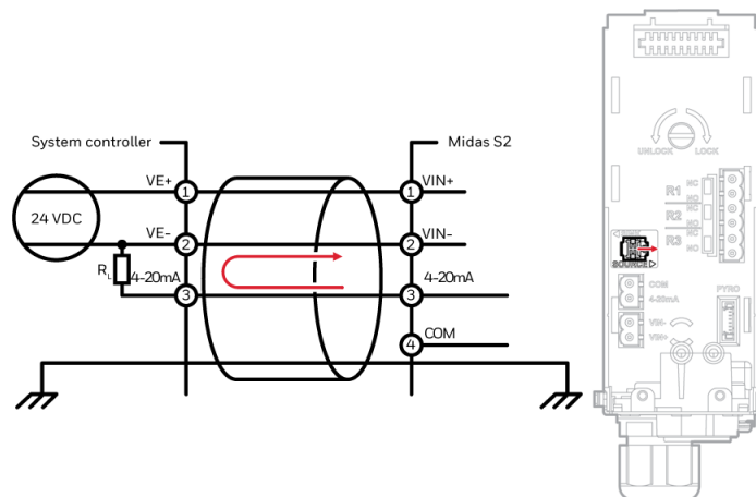
FIGURE 2 -3: Detector Source Mode with DC Power
