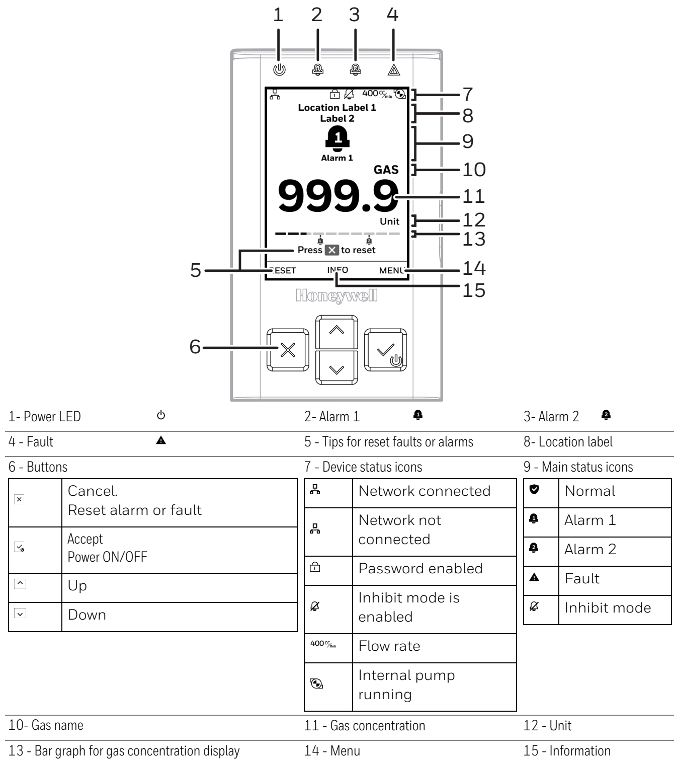
FIGURE 1 -2: Device's interface components
