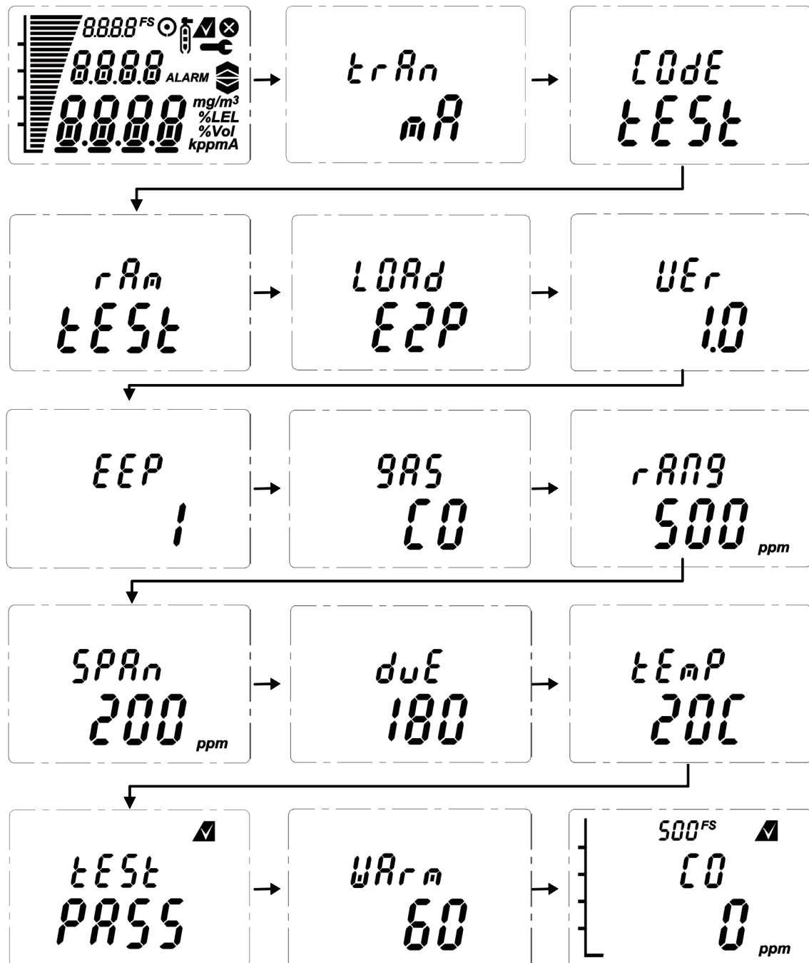
Diagram 14: Normal Start up procedure (For the CO sensor version)
