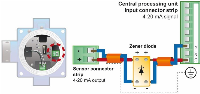
Figure 9: connection for an intrinsically safe, 2-wire 4-20 Ma detector with a Zener diode 024
