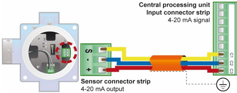
Figure 10: connection for a 3-wire 4-20 Ma detector 023
