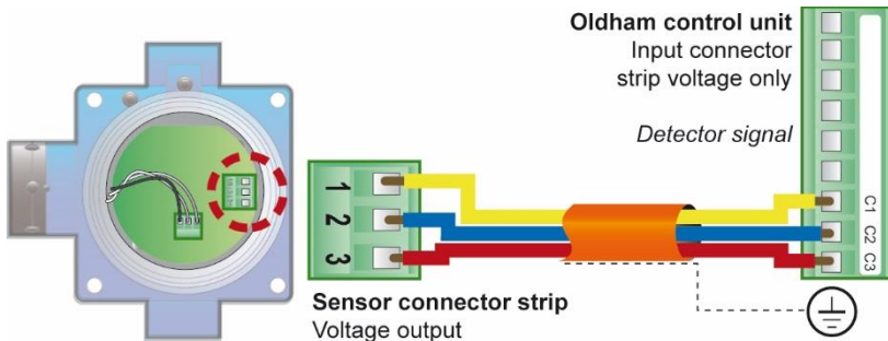
Figure 11: connection for a 3-wire OLC 100 type detector 026
