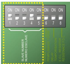
Figure 4: Switches for address configuration
