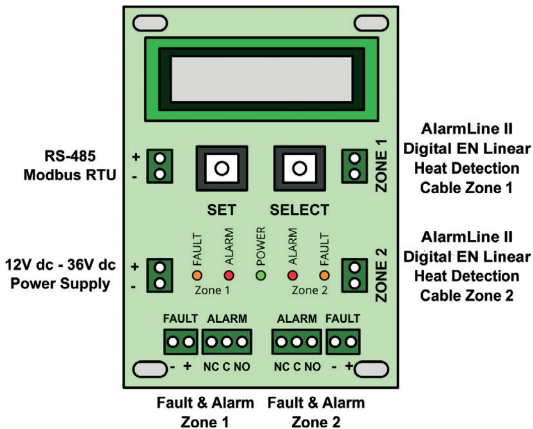
Figure 3: Wiring Diagram for the Kidde AlarmLine II Digital EN Controller
