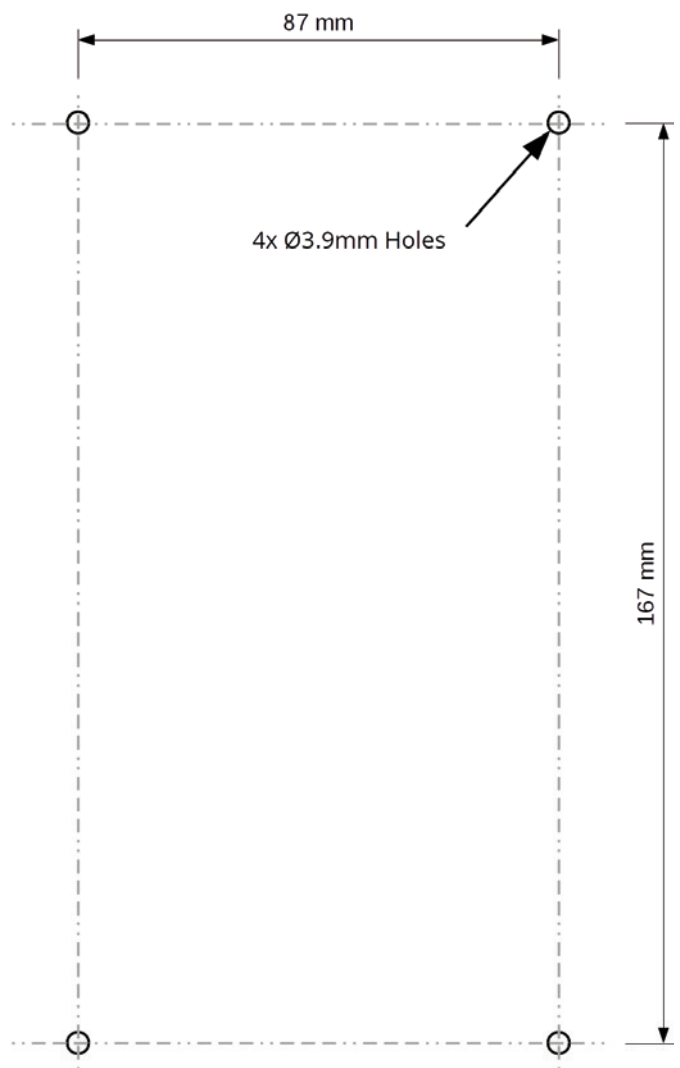
Figure 2: Mounting Dimensions for the Kidde AlarmLine II Digital EN Controller
