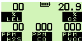
Fig. 2.10 Acknowledge Alarm
